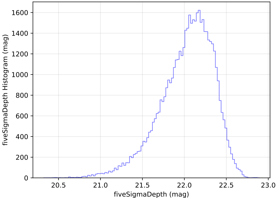
ddf_loaded_fl15_v3.4_10yrs Yr 1 y band: fiveSigmaDepth Histogram
