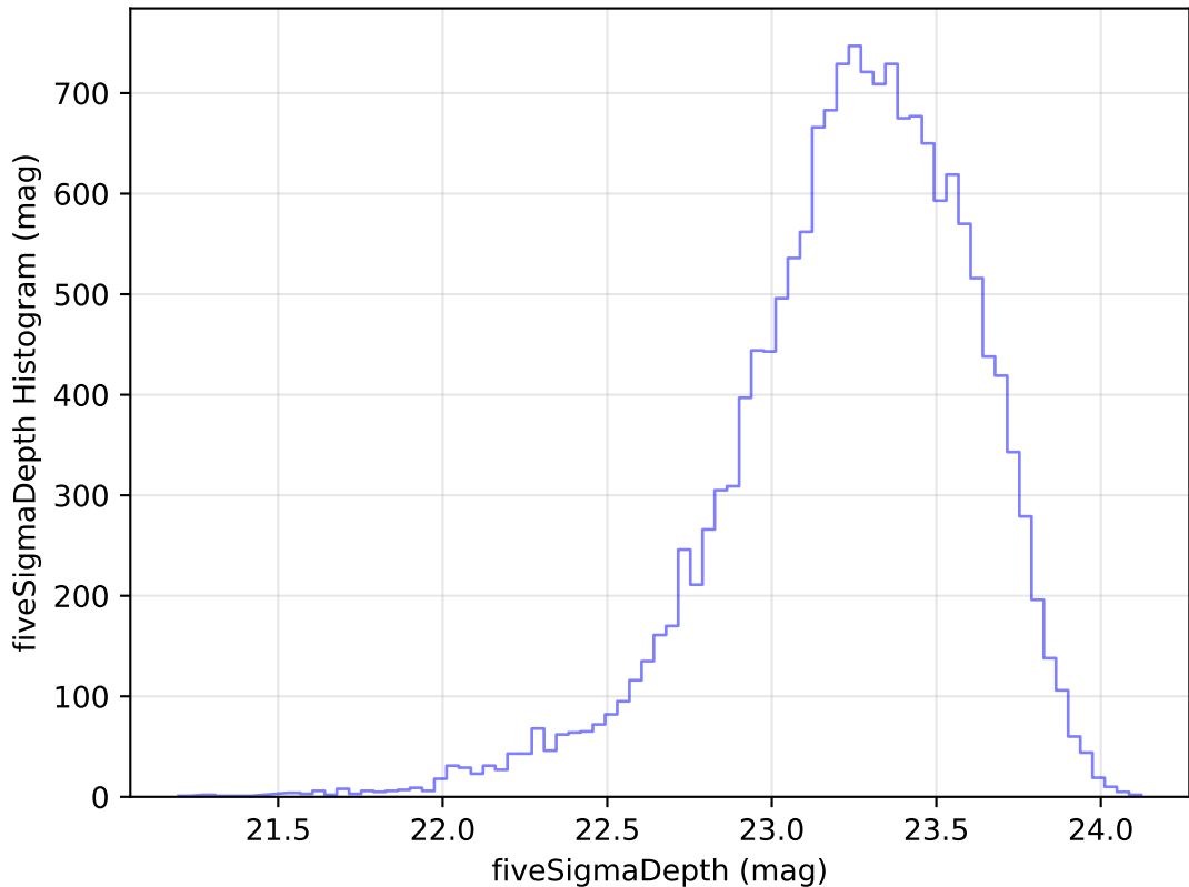
ddf_loaded_fl15_v3.4_10yrs Yr 1 u band: fiveSigmaDepth Histogram
