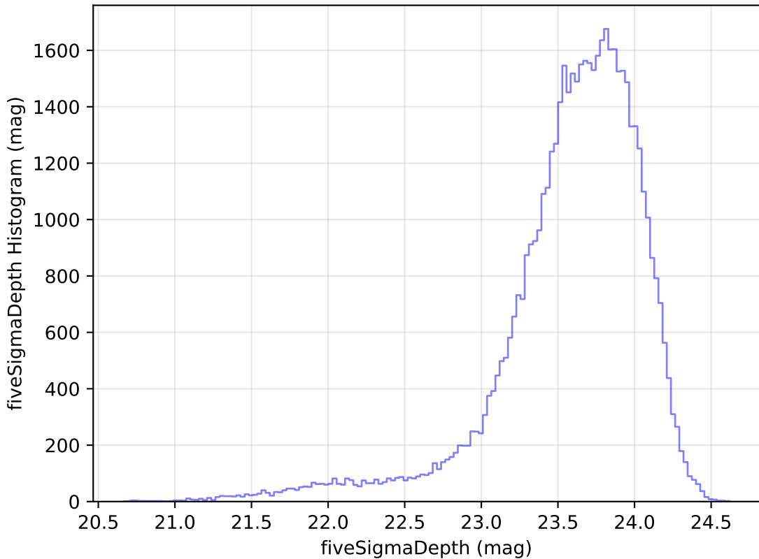
ddf_loaded_fl15_v3.4_10yrs Yr 1 i band: fiveSigmaDepth Histogram
