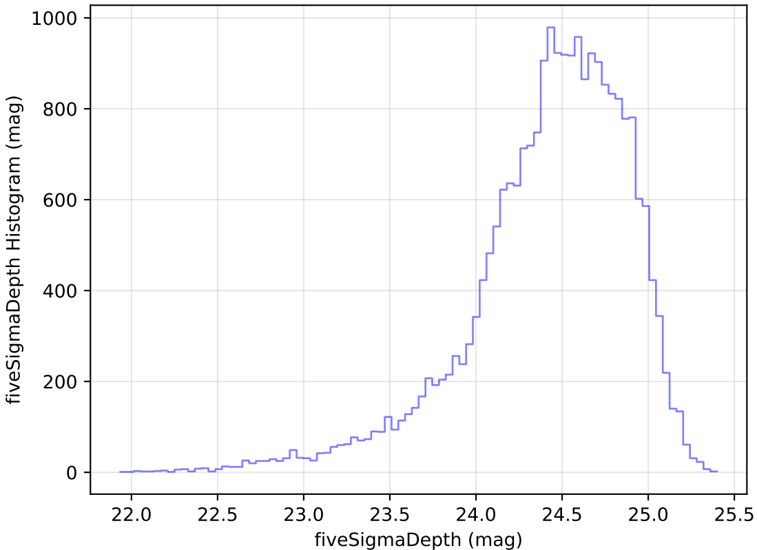
ddf_loaded_fl15_v3.4_10yrs Yr 1 g band: fiveSigmaDepth Histogram
