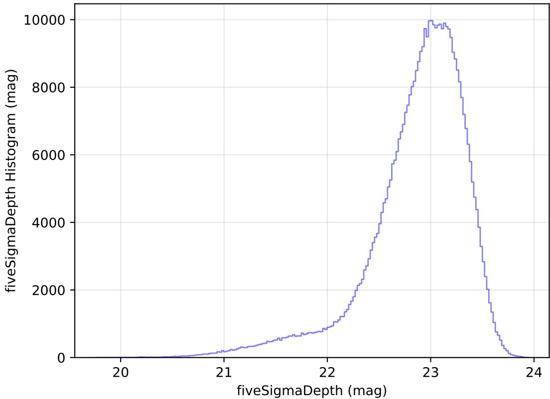
ddf_loaded_fl15_v3.4_10yrs WFD z band: fiveSigmaDepth Histogram
