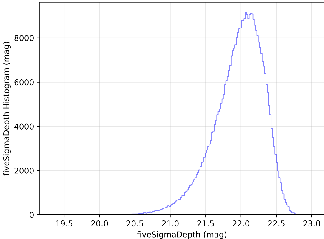
ddf_loaded_fl15_v3.4_10yrs WFD y band: fiveSigmaDepth Histogram
