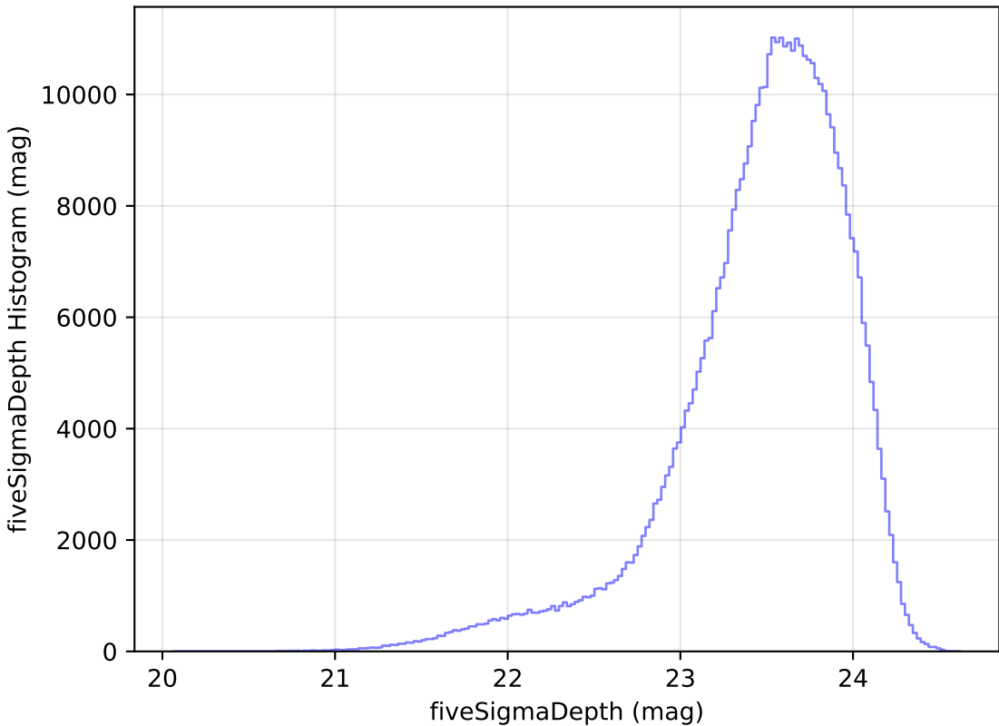
ddf_loaded_fl15_v3.4_10yrs WFD i band: fiveSigmaDepth Histogram
