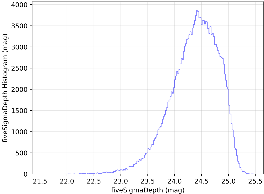
ddf_loaded_fl15_v3.4_10yrs WFD g band: fiveSigmaDepth Histogram
