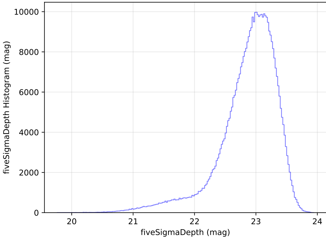
ddf_loaded_fl15_v3.4_10yrs All sky z band: fiveSigmaDepth Histogram
