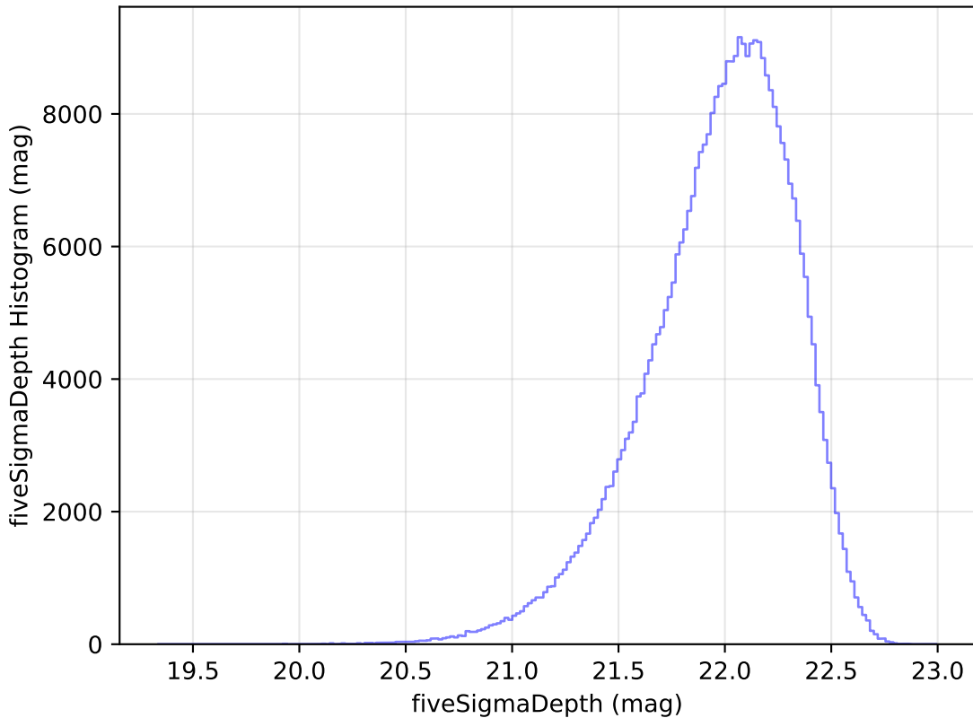
ddf_loaded_fl15_v3.4_10yrs All sky y band: fiveSigmaDepth Histogram
