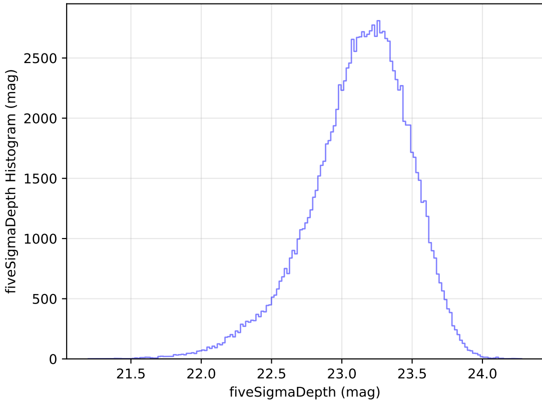
ddf_loaded_fl15_v3.4_10yrs All sky u band: fiveSigmaDepth Histogram
