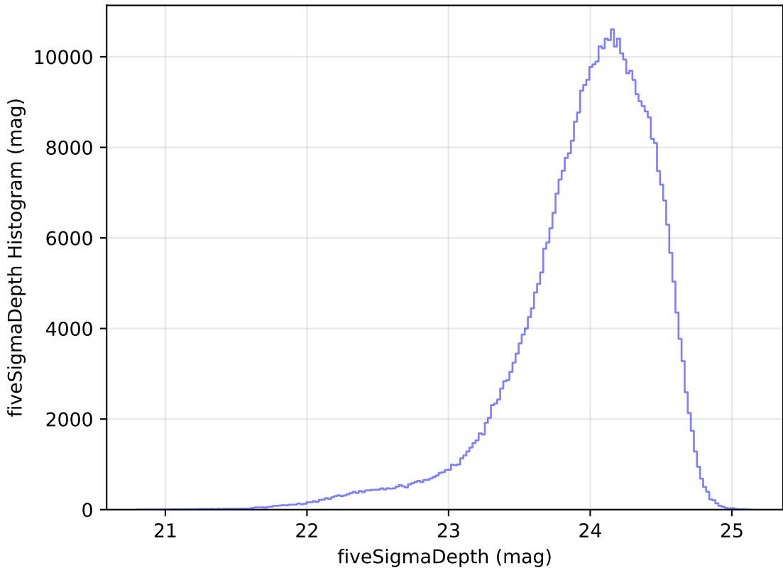
ddf_loaded_fl15_v3.4_10yrs All sky r band: fiveSigmaDepth Histogram
