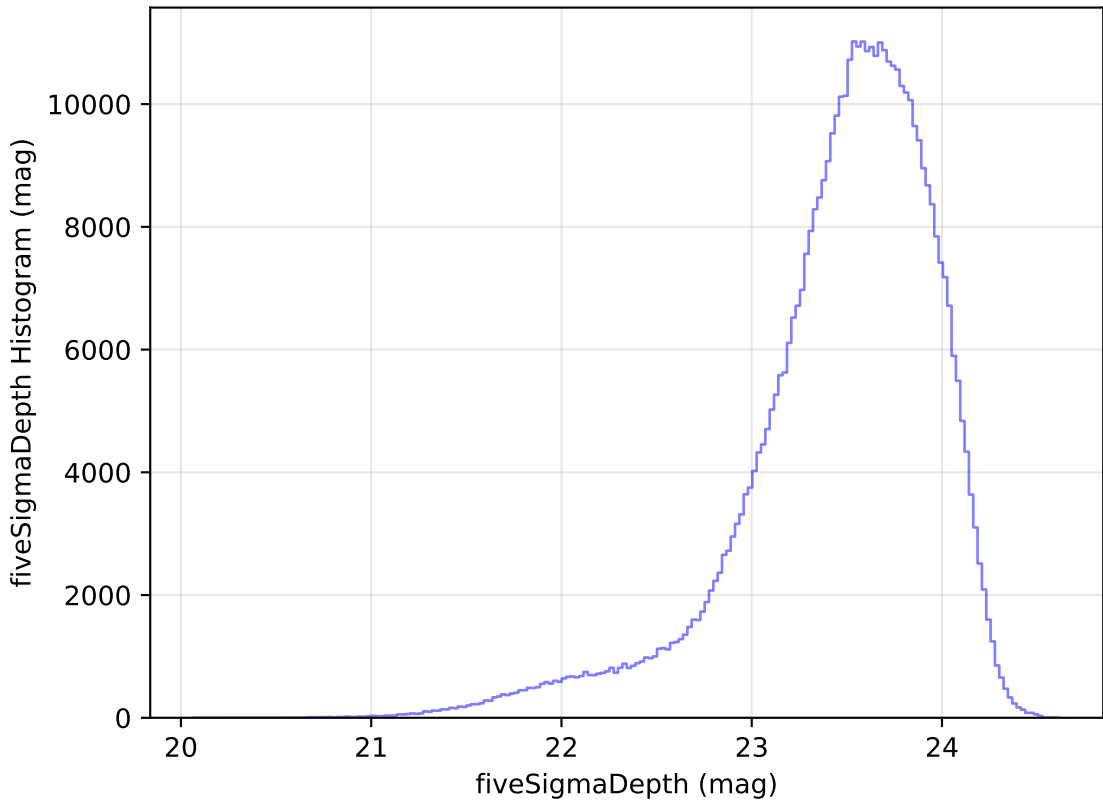
ddf_loaded_fl15_v3.4_10yrs All sky i band: fiveSigmaDepth Histogram
