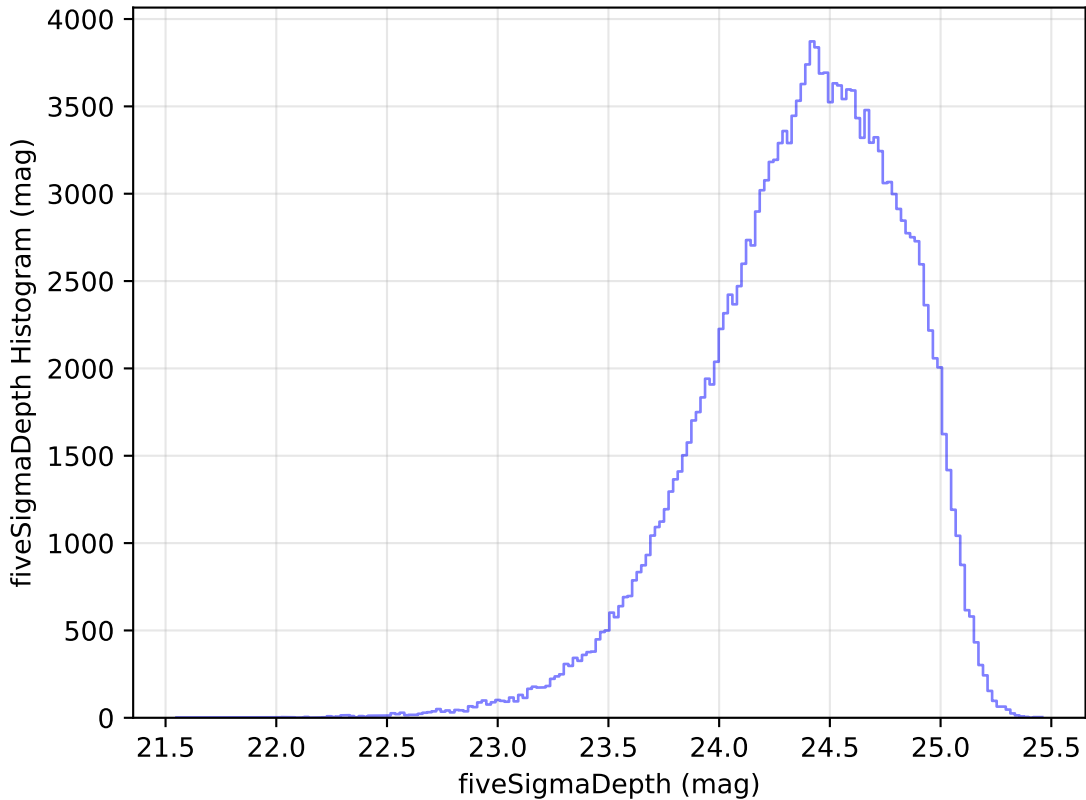
ddf_loaded_fl15_v3.4_10yrs All sky g band: fiveSigmaDepth Histogram
