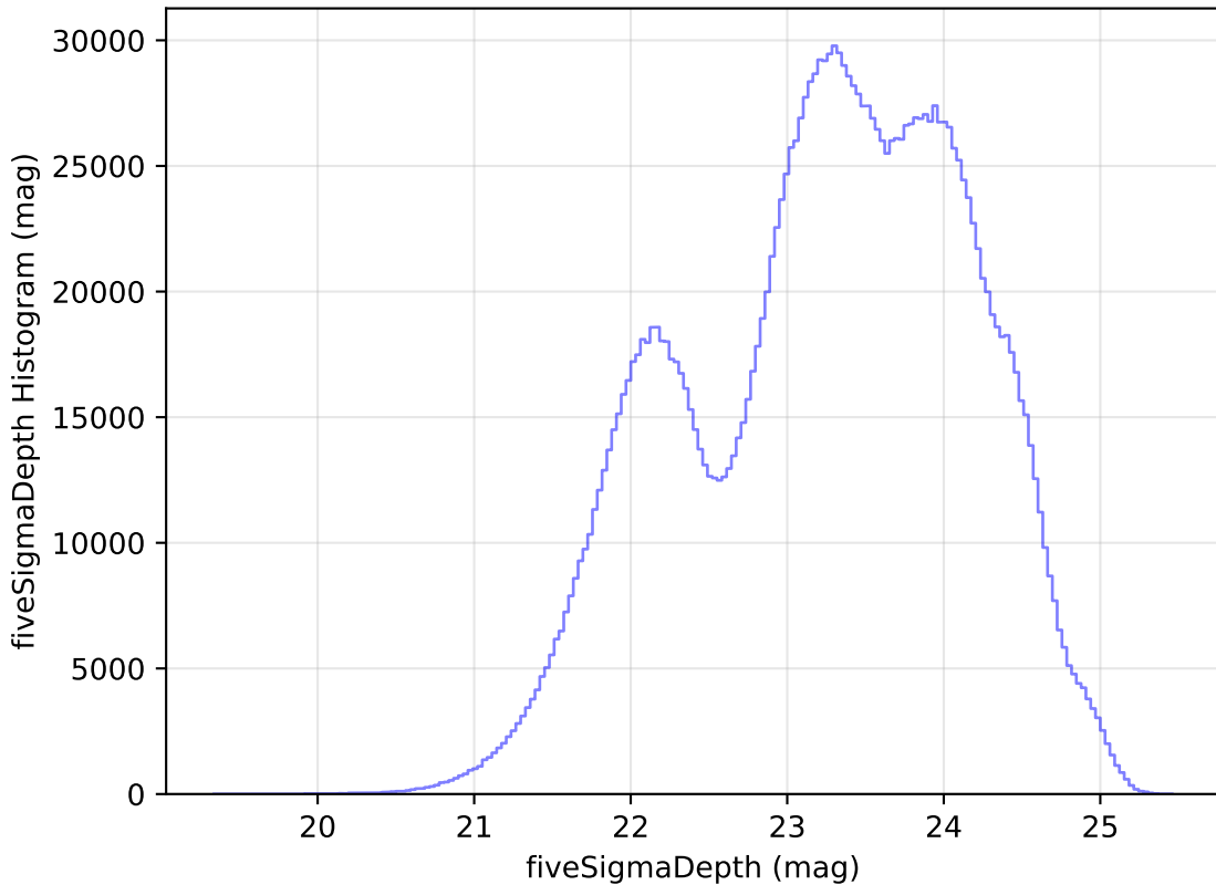
ddf_loaded_fl15_v3.4_10yrs All sky all bands: fiveSigmaDepth Histogram
