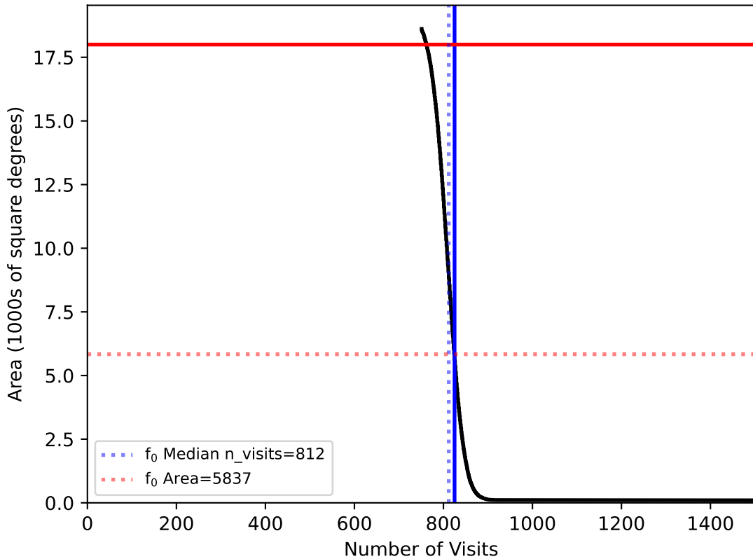
ddf_loaded_fl15_v3.4_10yrs WFD: fO
