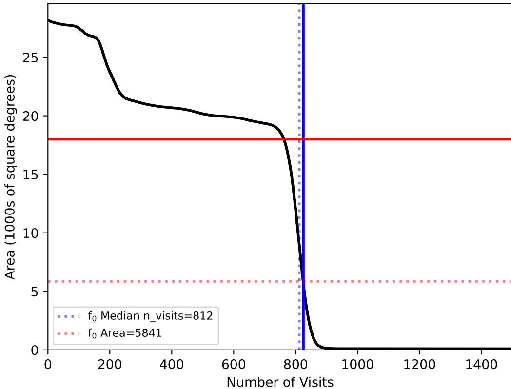
ddf_loaded_fl15_v3.4_10yrs All sky: fO
