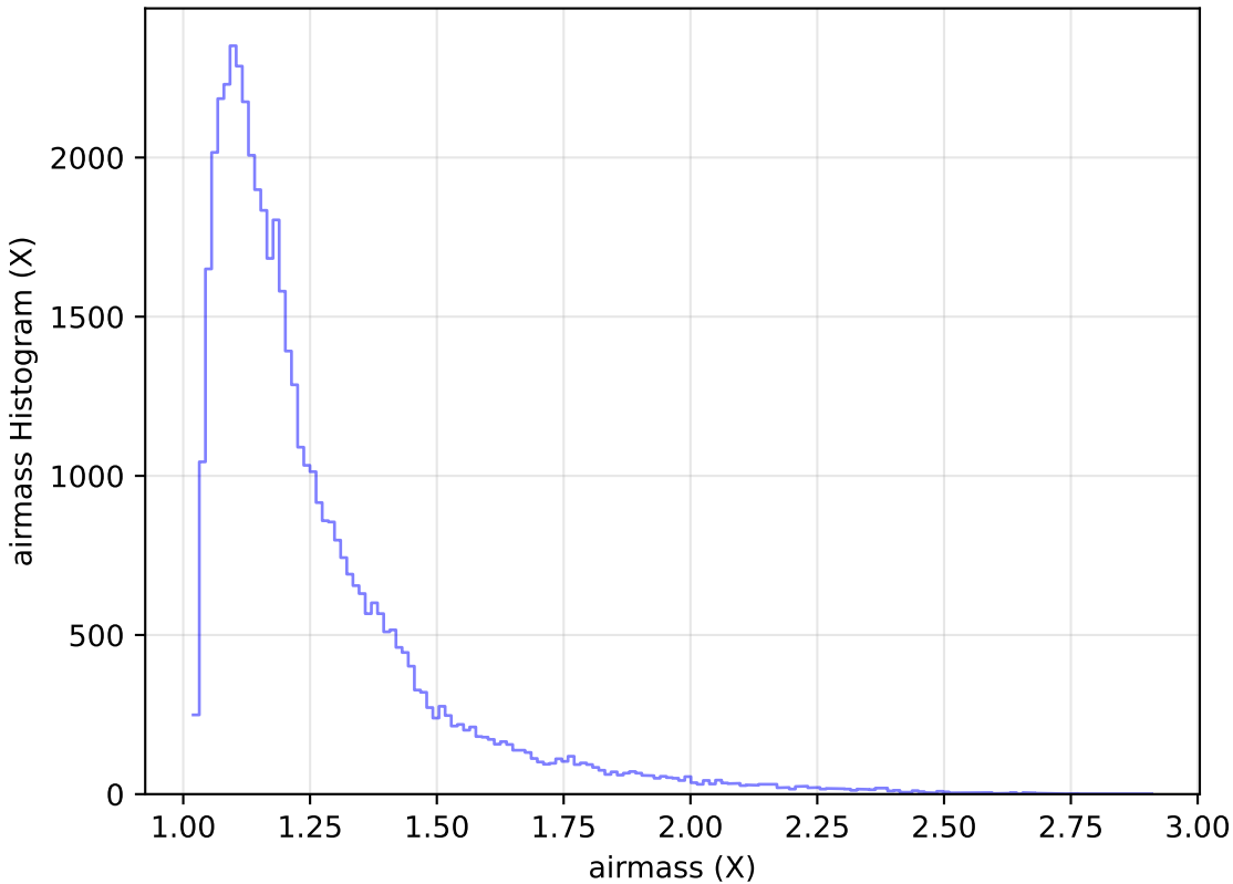
ddf_loaded_fl15_v3.4_10yrs Yr 1 y band: airmass Histogram
