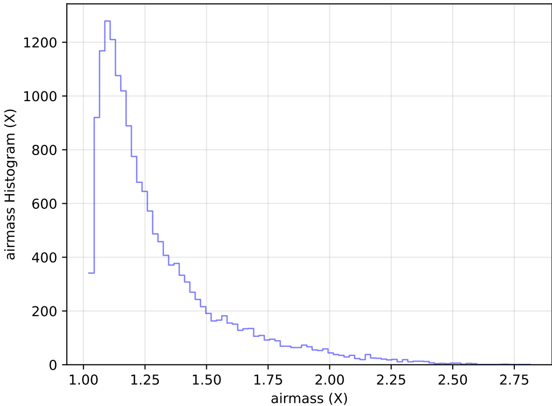
ddf_loaded_fl15_v3.4_10yrs Yr 1 u band: airmass Histogram
