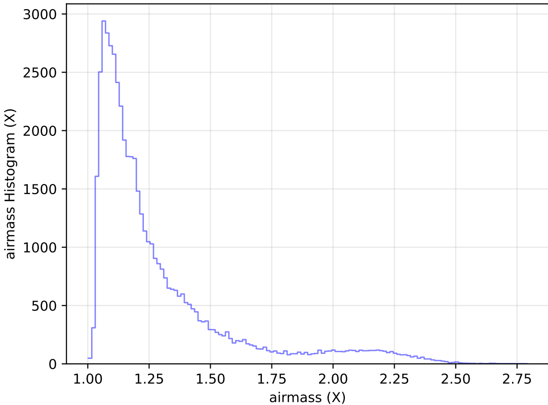
ddf_loaded_fl15_v3.4_10yrs Yr 1 r band: airmass Histogram
