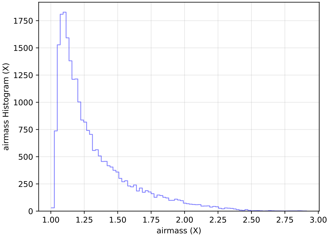
ddf_loaded_fl15_v3.4_10yrs Yr 1 g band: airmass Histogram
