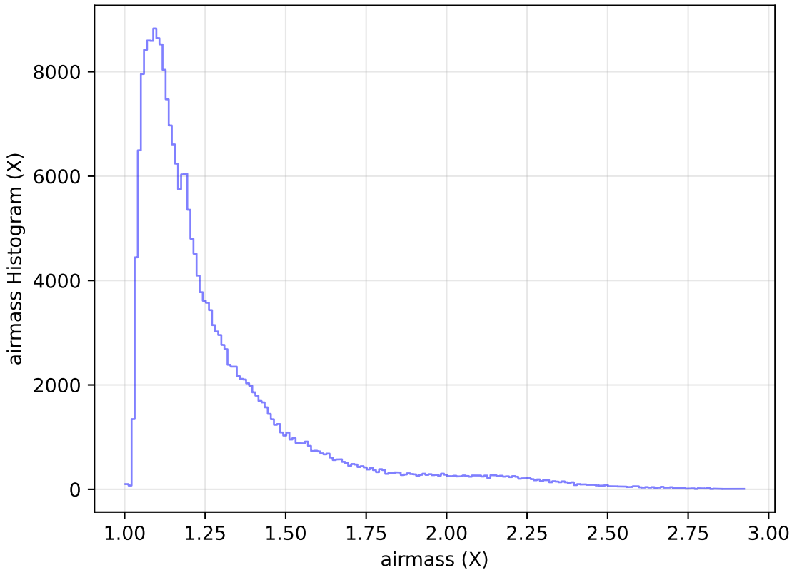
ddf_loaded_fl15_v3.4_10yrs Yr 1 all bands: airmass Histogram
