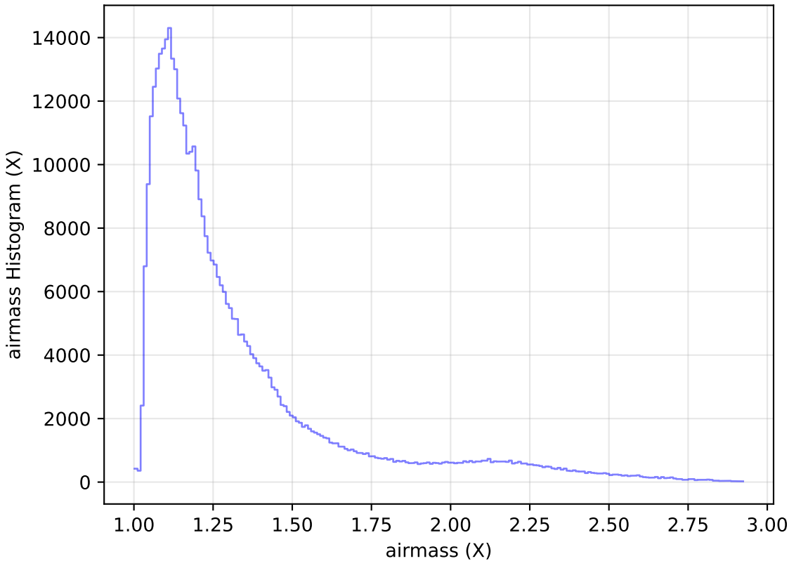
ddf_loaded_fl15_v3.4_10yrs WFD z band: airmass Histogram
