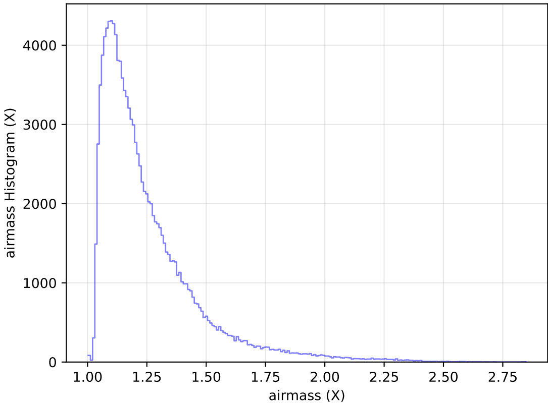
ddf_loaded_fl15_v3.4_10yrs WFD u band: airmass Histogram
