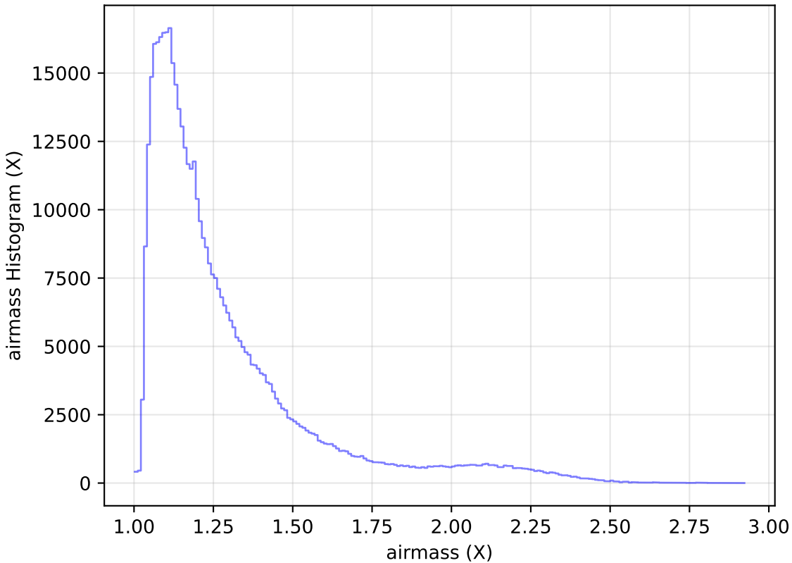
ddf_loaded_fl15_v3.4_10yrs WFD r band: airmass Histogram
