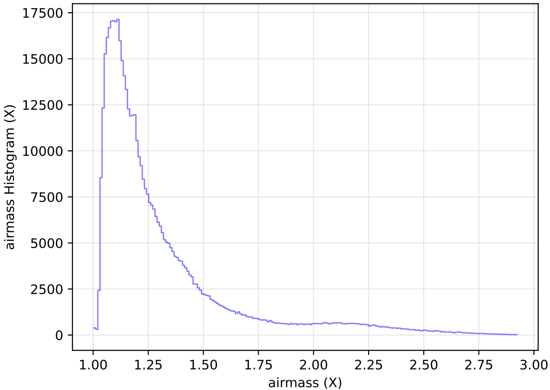
ddf_loaded_fl15_v3.4_10yrs WFD i band: airmass Histogram
