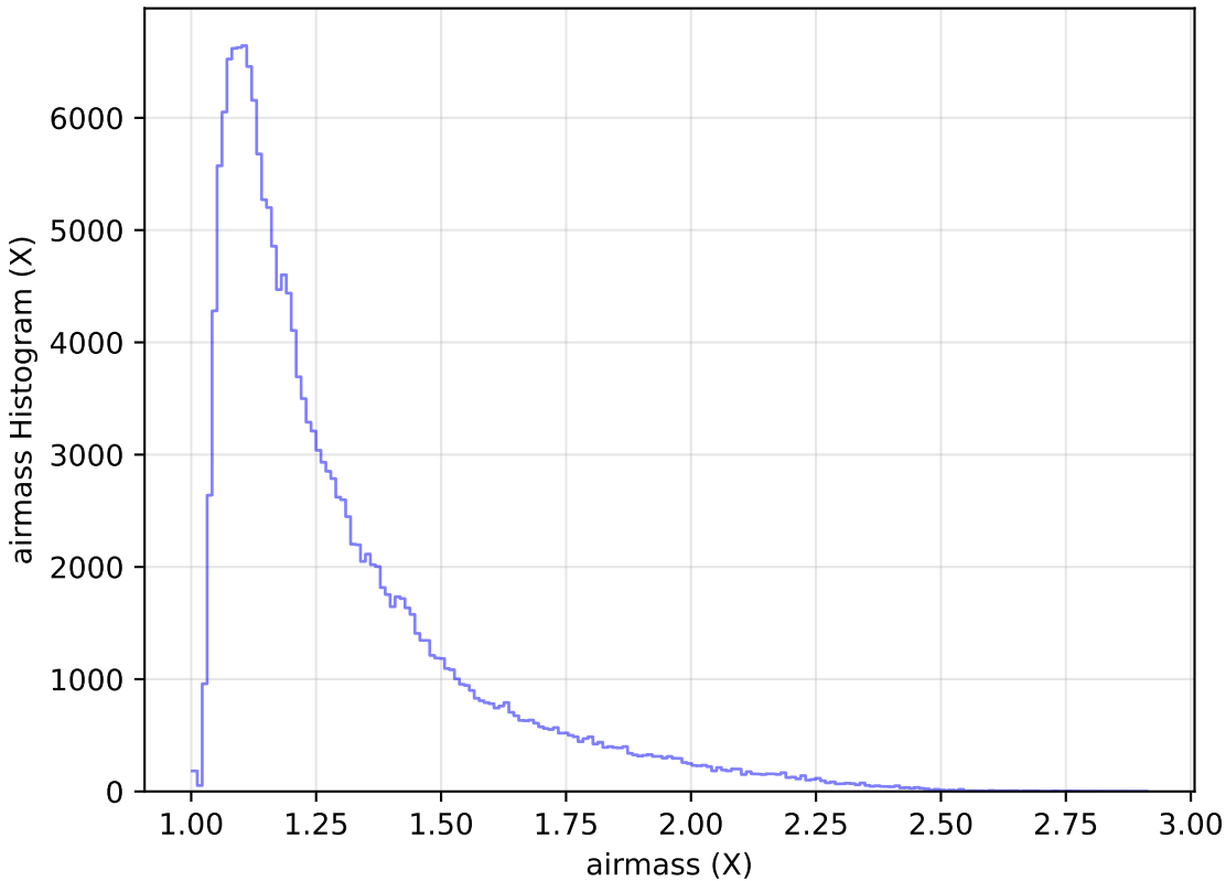
ddf_loaded_fl15_v3.4_10yrs WFD g band: airmass Histogram
