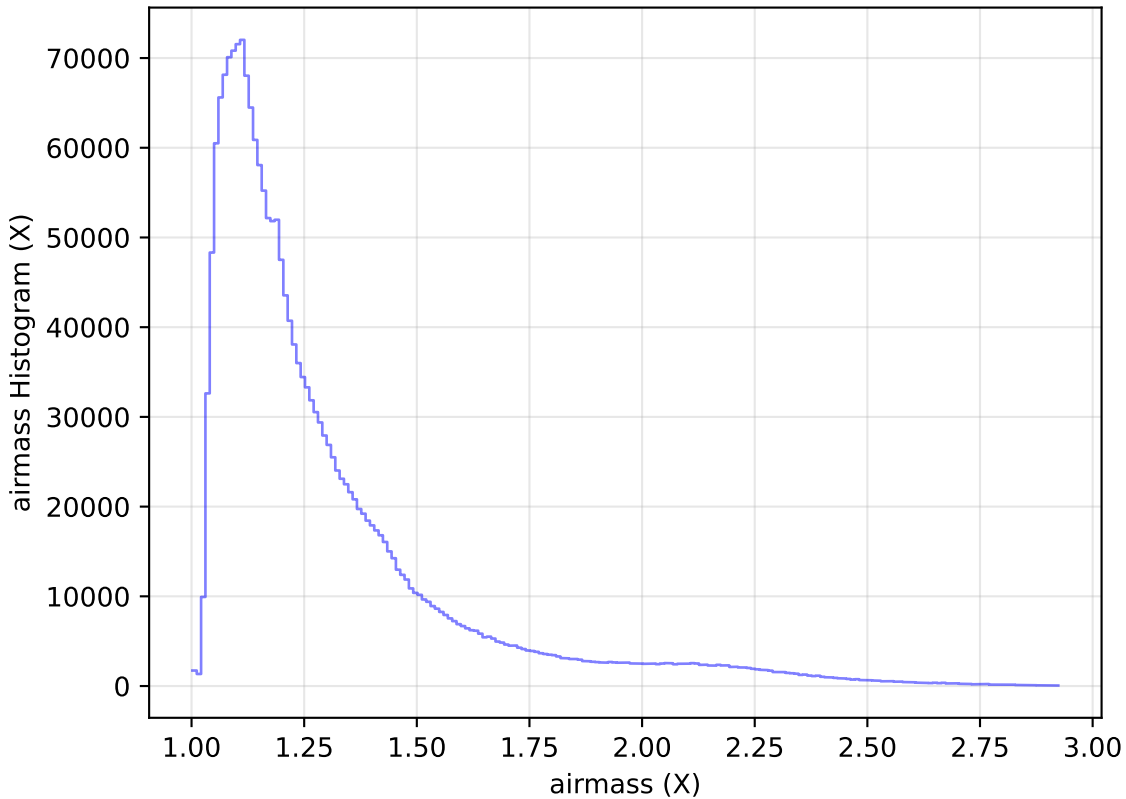
ddf_loaded_fl15_v3.4_10yrs WFD all bands: airmass Histogram
