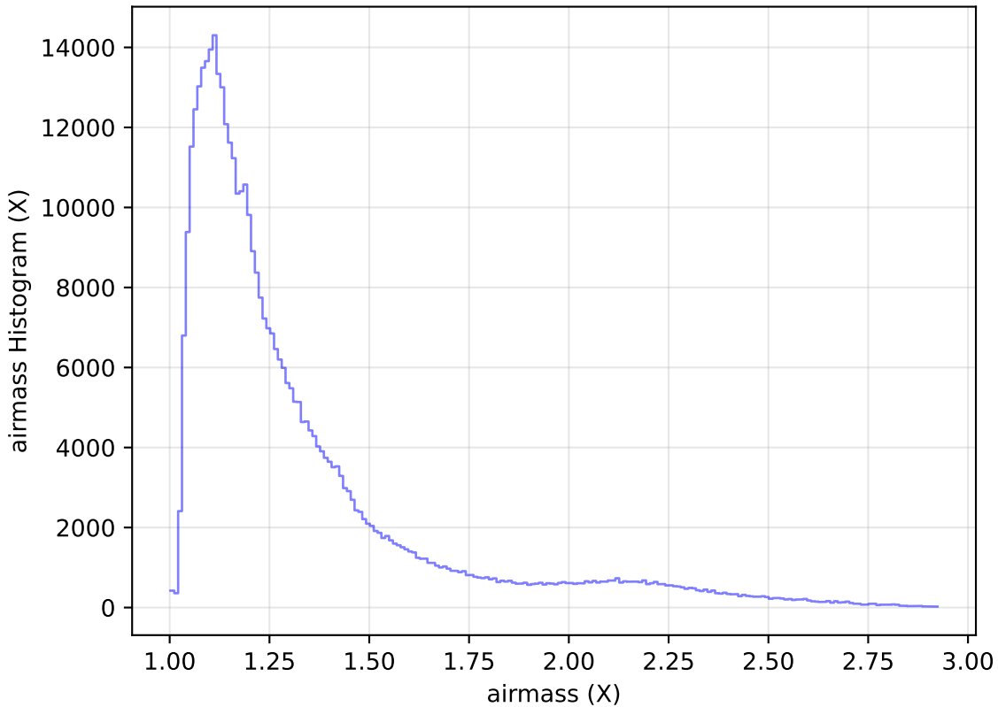
ddf_loaded_fl15_v3.4_10yrs All sky z band: airmass Histogram
