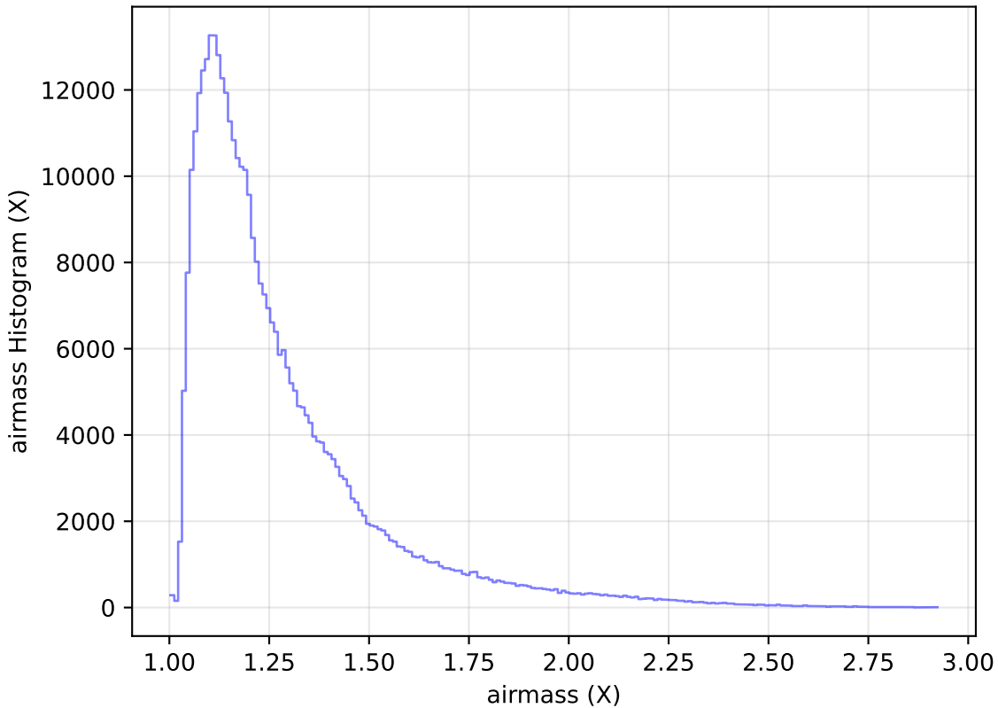
ddf_loaded_fl15_v3.4_10yrs All sky y band: airmass Histogram
