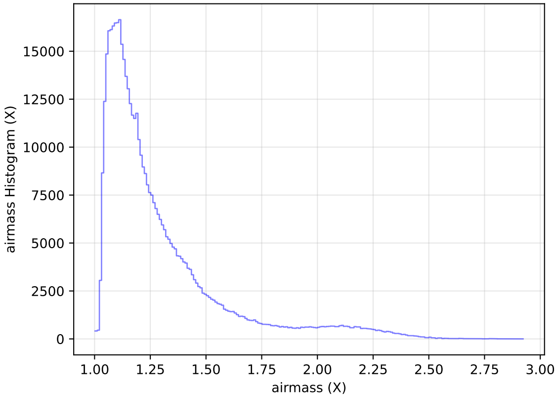
ddf_loaded_fl15_v3.4_10yrs All sky r band: airmass Histogram
