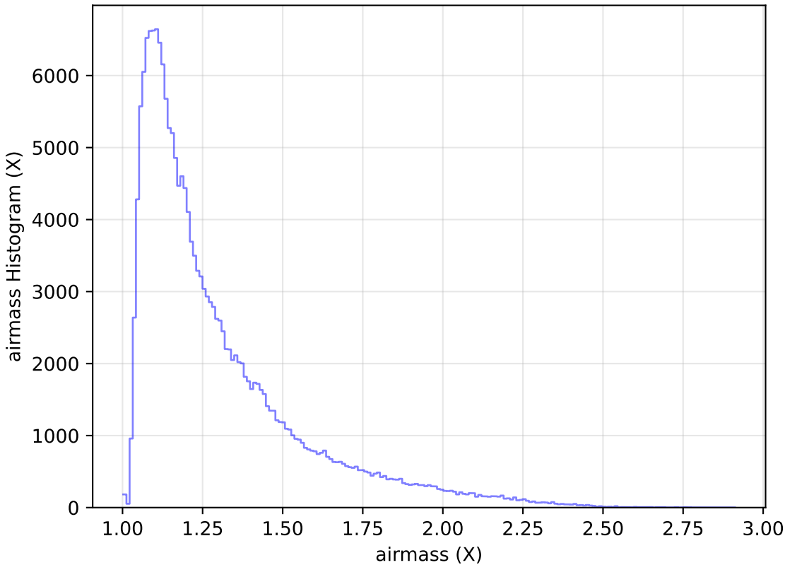
ddf_loaded_fl15_v3.4_10yrs All sky g band: airmass Histogram
