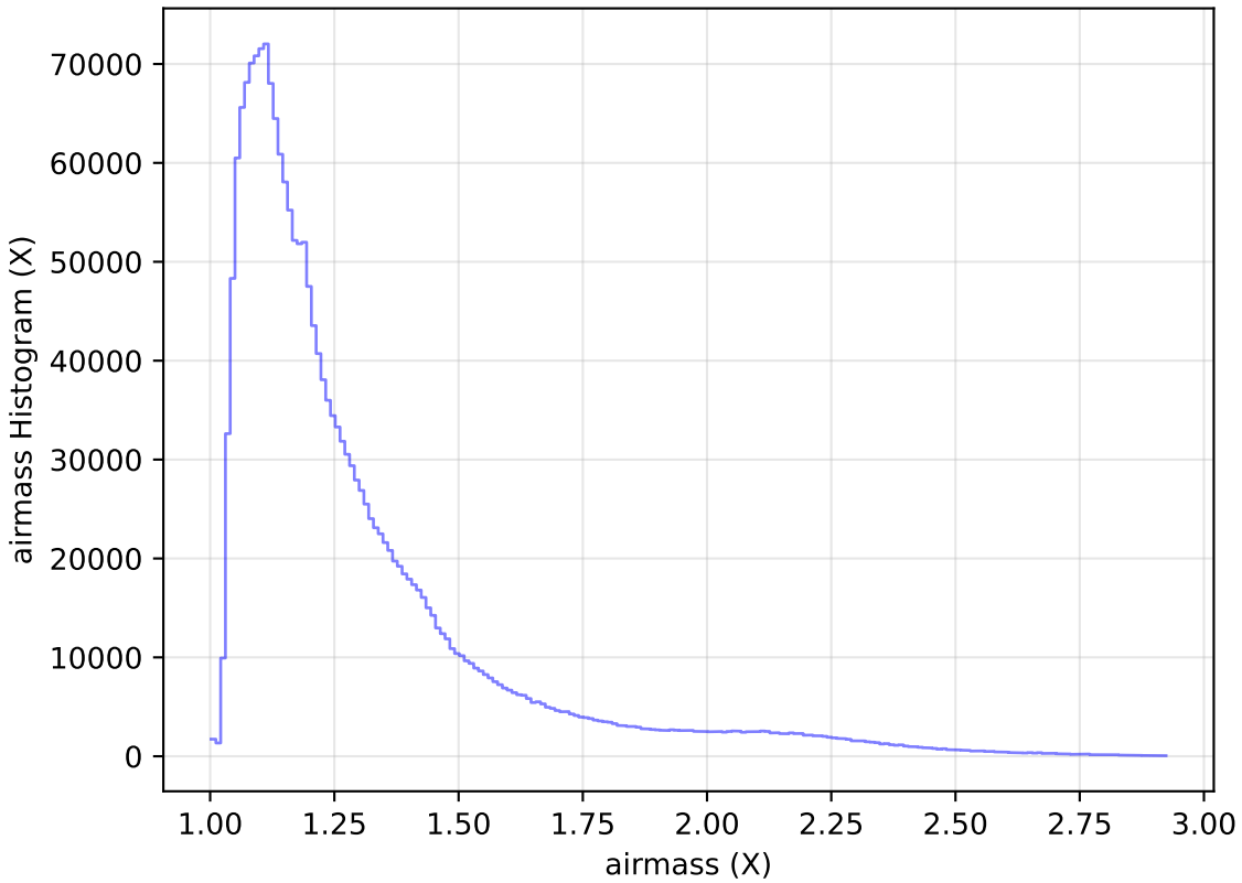
ddf_loaded_fl15_v3.4_10yrs All sky all bands: airmass Histogram
