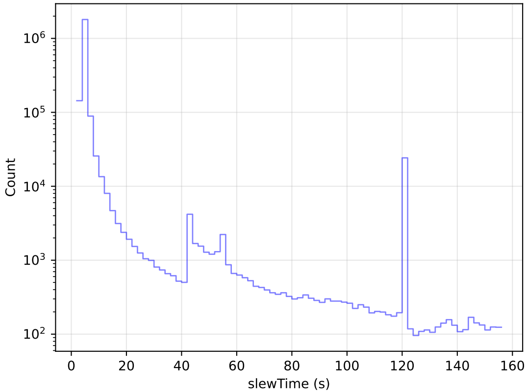
ddf_loaded_fl15_v3.4_10yrs All visits: Slew Time Histogram
