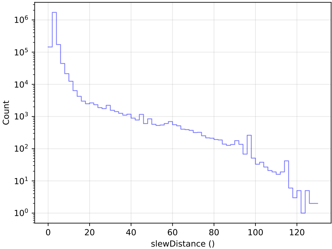
ddf_loaded_fl15_v3.4_10yrs All visits: Slew Distance Histogram
