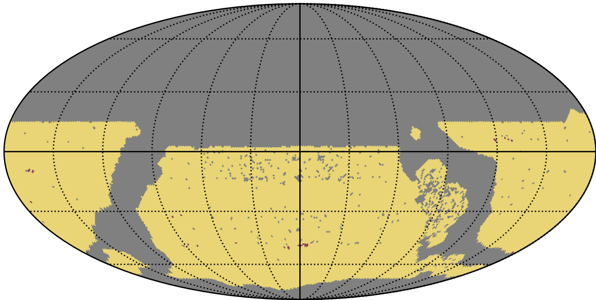
ddf_loaded_fl15_v3.4_10yrs WFD: RapidRevisits
