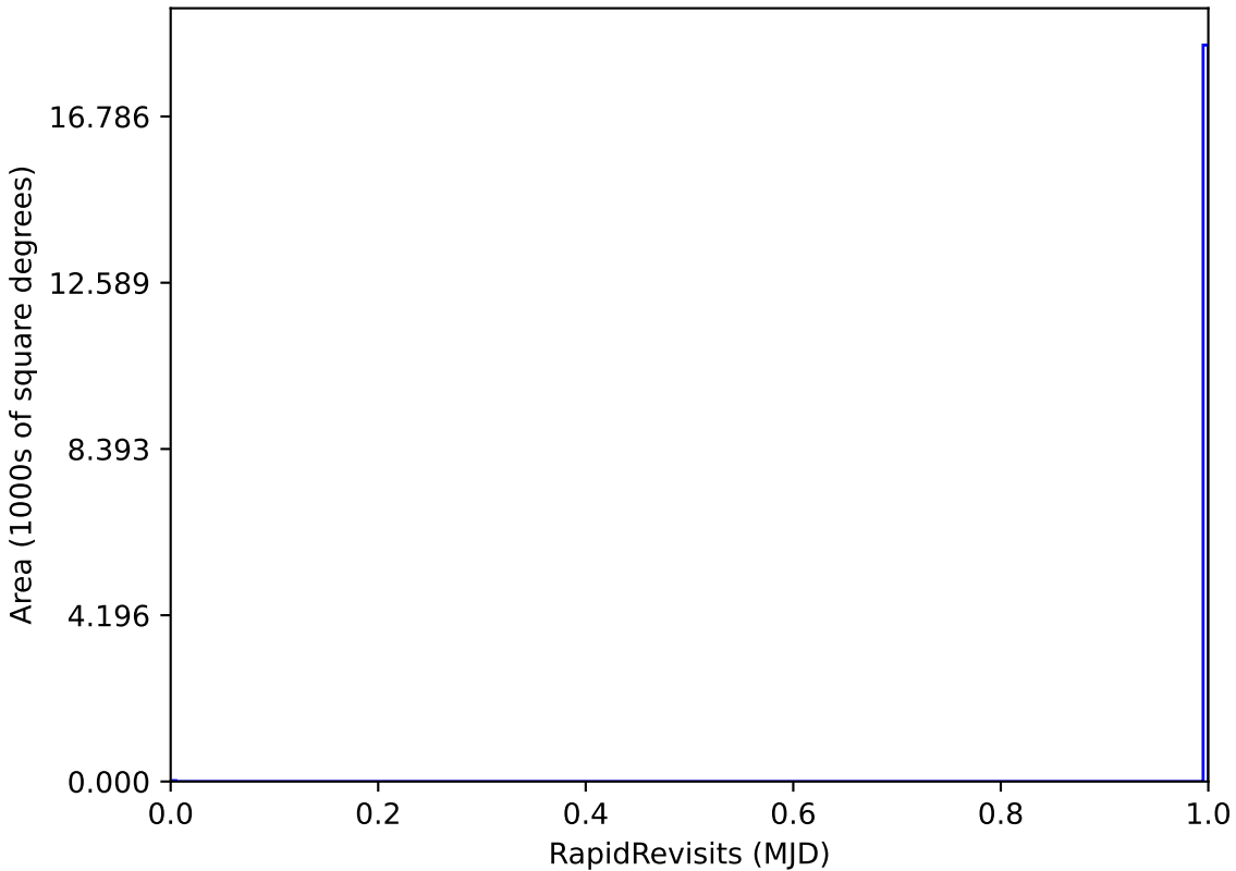
ddf_loaded_fl15_v3.4_10yrs WFD: RapidRevisits
