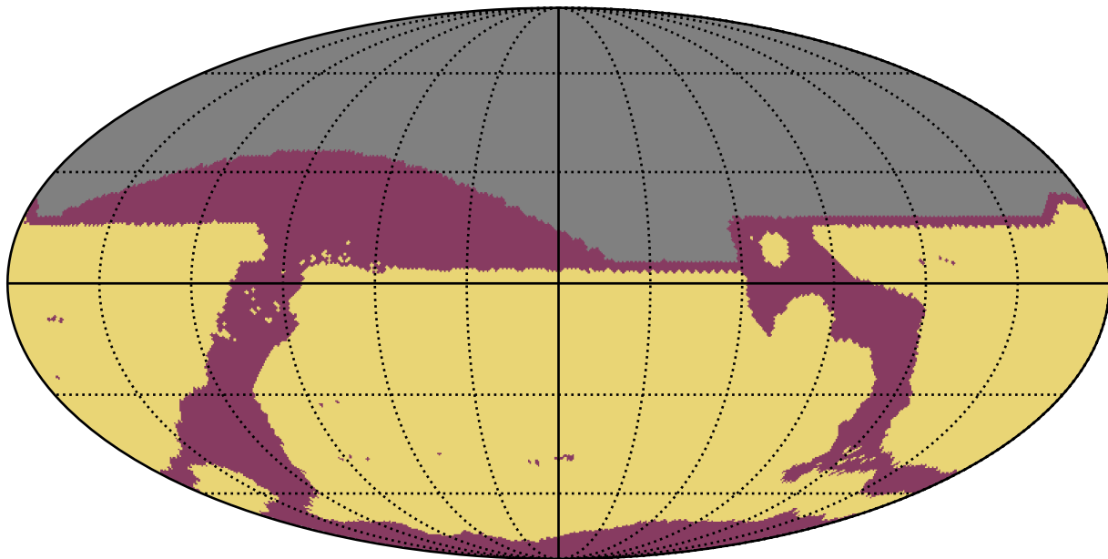
ddf_loaded_fl15_v3.4_10yrs All sky: RapidRevisits
