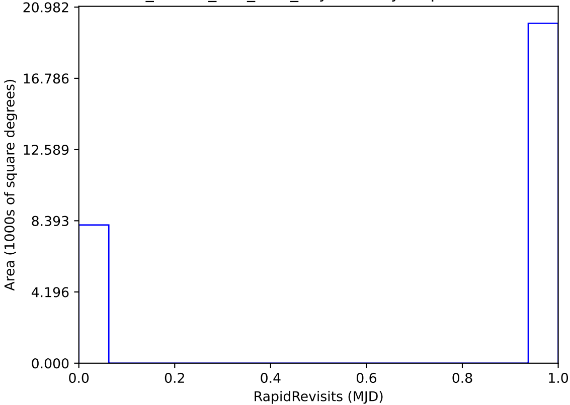
ddf_loaded_fl15_v3.4_10yrs All sky: RapidRevisits
