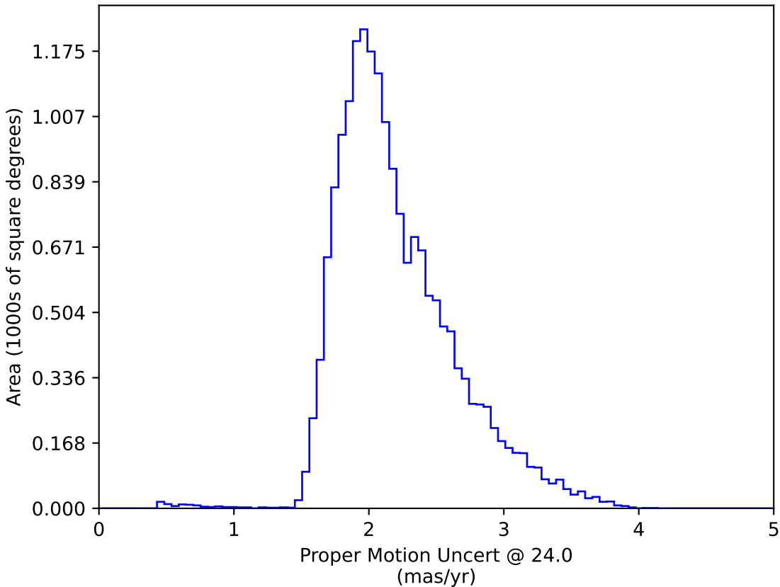
ddf_loaded_fl15_v3.4_10yrs WFD: Proper Motion Uncert @ 24.0
