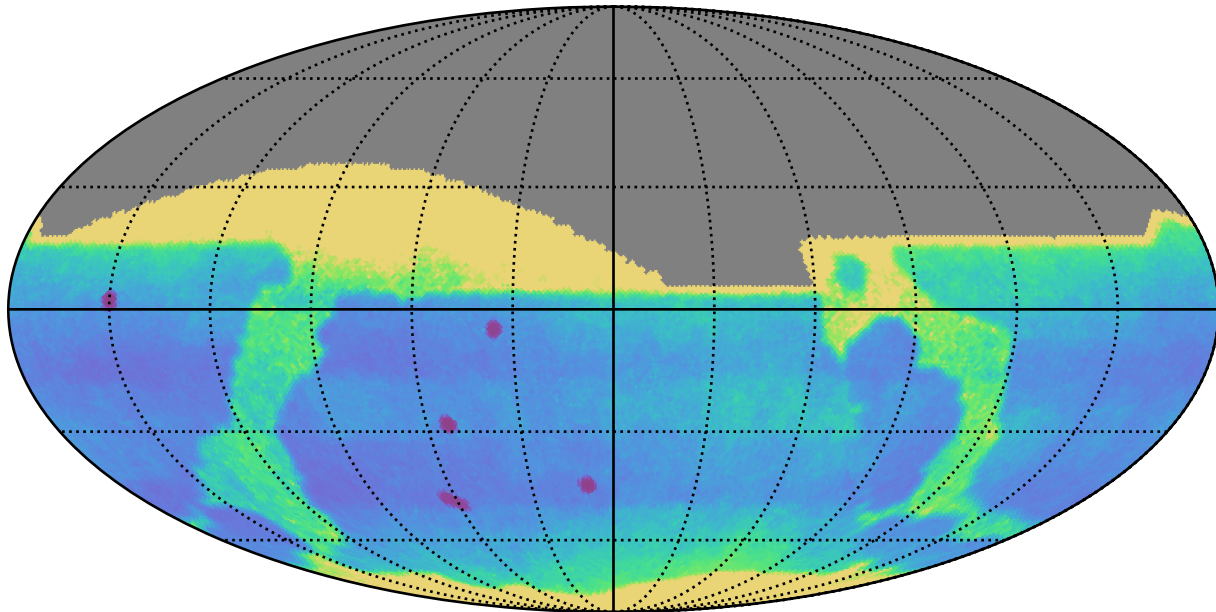
ddf_loaded_fl15_v3.4_10yrs All sky: Proper Motion Uncert @ 24.0
