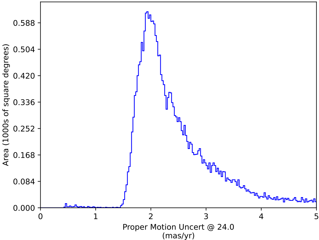
ddf_loaded_fl15_v3.4_10yrs All sky: Proper Motion Uncert @ 24.0
