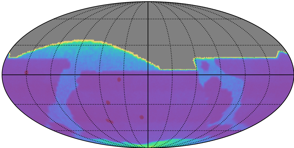
ddf_loaded_fl15_v3.4_10yrs All sky: Proper Motion Uncert @ 20.5
