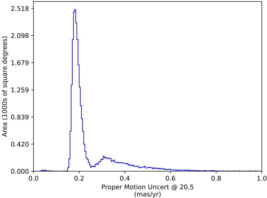
ddf_loaded_fl15_v3.4_10yrs All sky: Proper Motion Uncert @ 20.5
