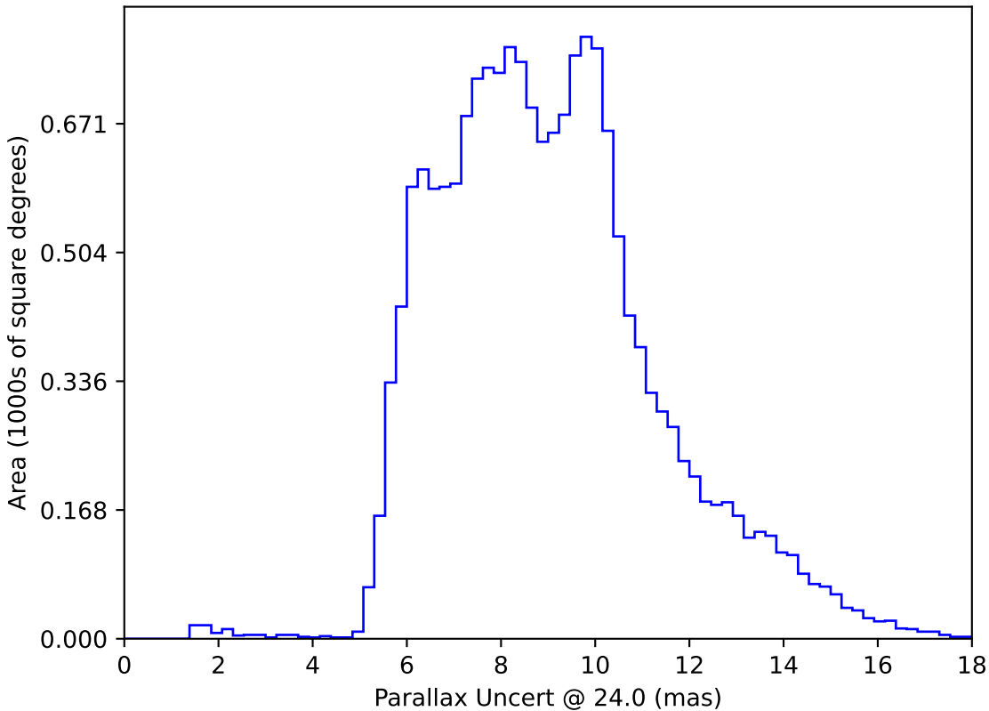
ddf_loaded_fl15_v3.4_10yrs WFD: Parallax Uncert @ 24.0
