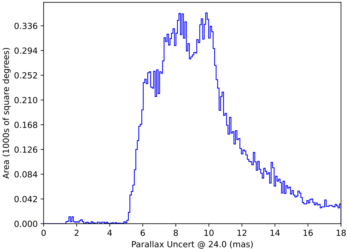
ddf_loaded_fl15_v3.4_10yrs All sky: Parallax Uncert @ 24.0
