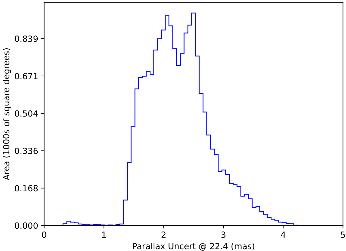
ddf_loaded_fl15_v3.4_10yrs WFD: Parallax Uncert @ 22.4
