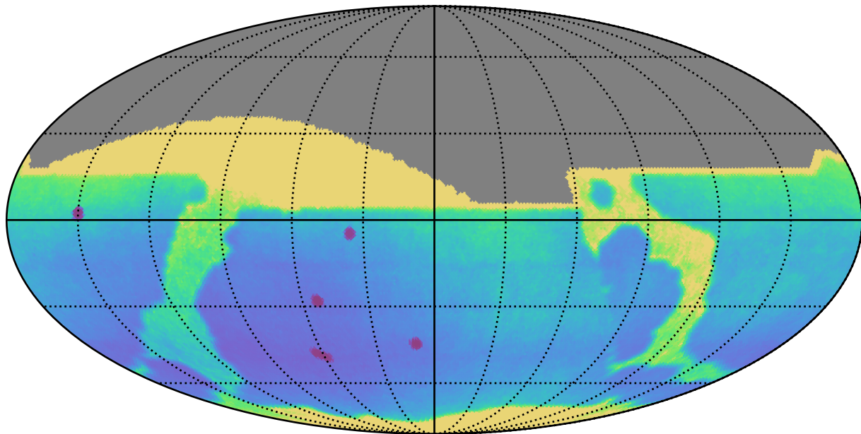
ddf_loaded_fl15_v3.4_10yrs All sky: Parallax Uncert @ 22.4
