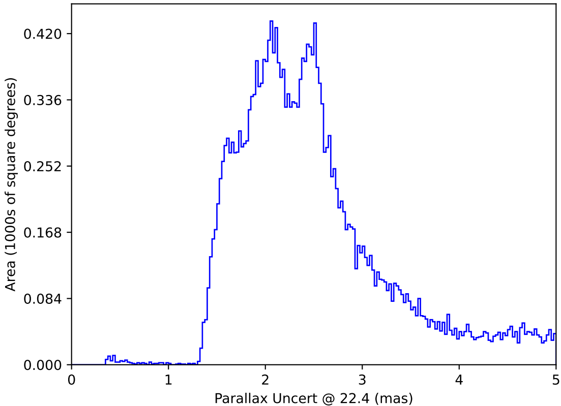
ddf_loaded_fl15_v3.4_10yrs All sky: Parallax Uncert @ 22.4
