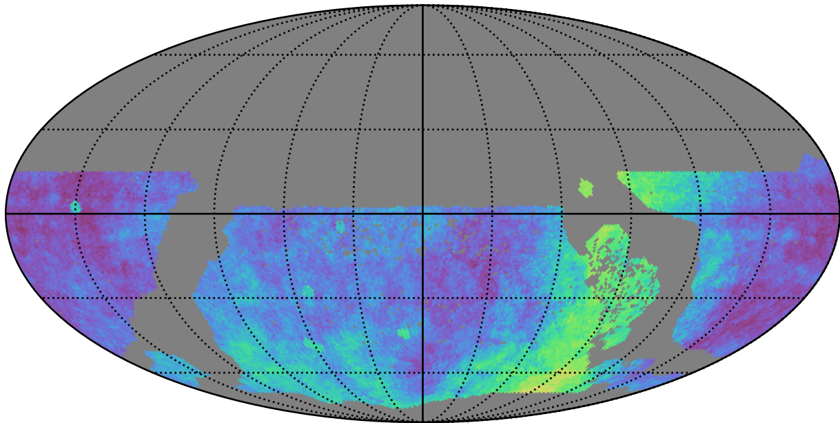
ddf_loaded_fl15_v3.4_10yrs WFD: Parallax Coverage @ 24.0
